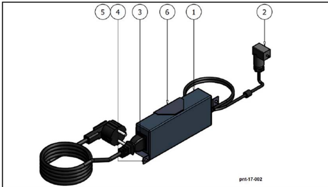
Figure 3.2; Overview components power adaptor
